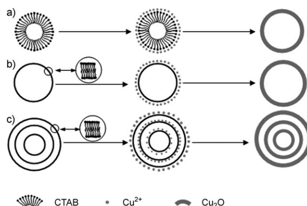
Scheme 1. The formation of different Cu 2 O hollow structures in the presence of a CTAB template: a) micelle, b) single-lamellar vesicle, c) multilamellar vesicle.
